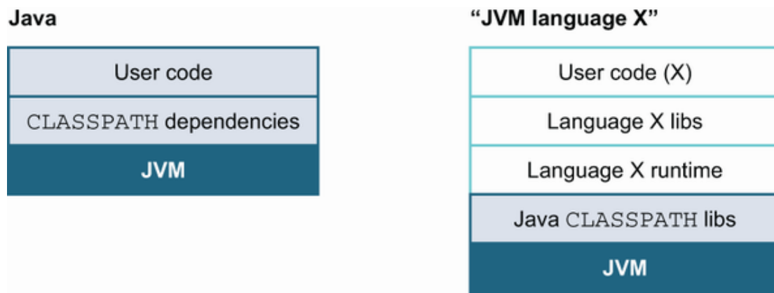
Figure 8.3 Non-Java language runtime support
