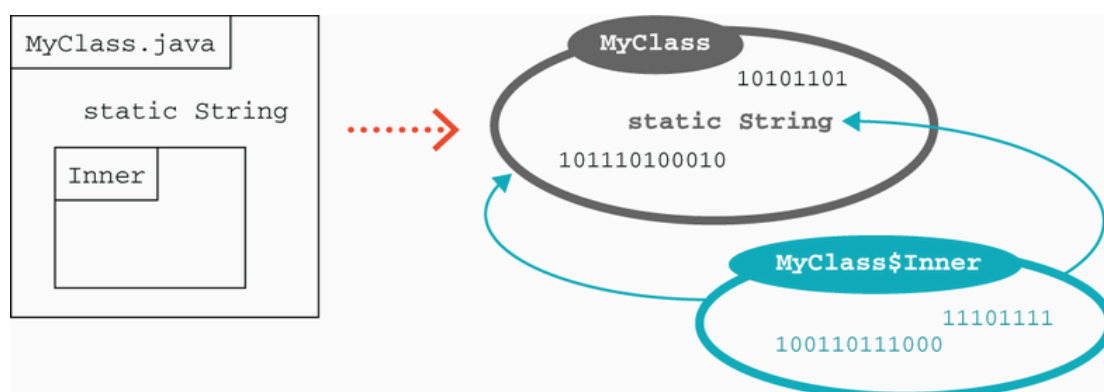
Figure 8.4 Inner classes as a compiler fiction
