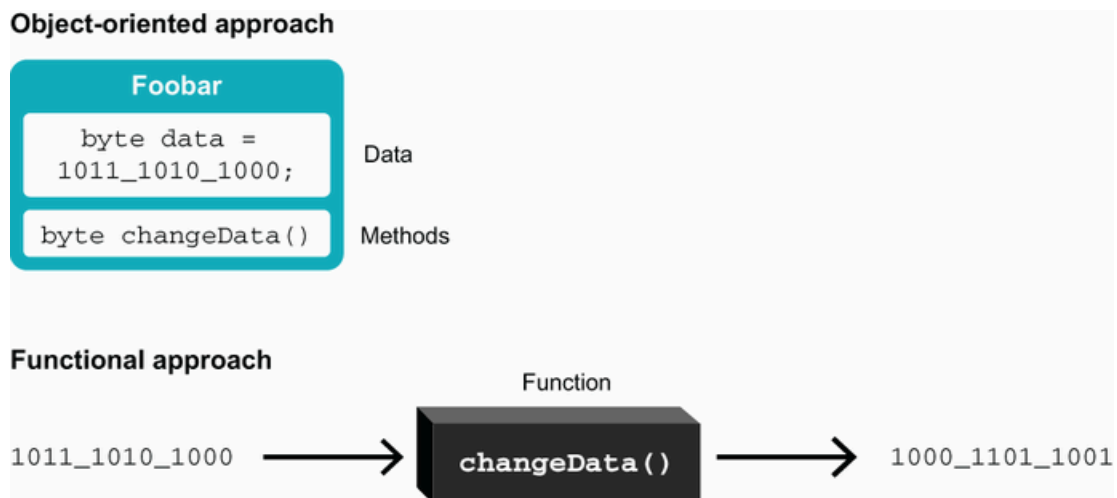
Figure 8.1 Imperative and functional languages
